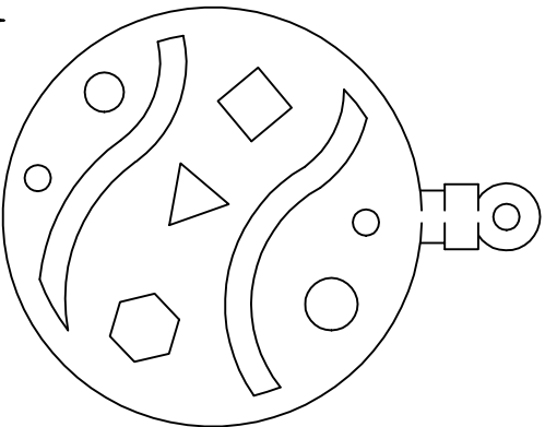
1 ORNAMENT 1 QTY.: 1 SIZE: 1/8" x 2 1/2" x 3"
